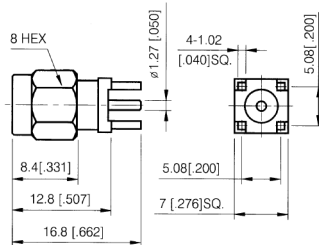
STRAIGHT PLUG FOR PRINTED CIRCUIT BOARD PART NUMBER 705487-001SMA
