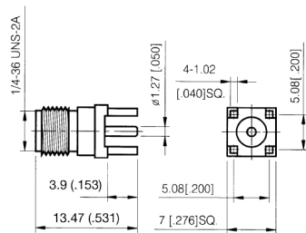
STRAIGHT JACK FOR PRINTED CIRCUIT BOARD PART NUMBER 705433-001SMA
