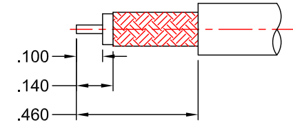
RECOMMENDED STRIPPING DIMENSIONS
