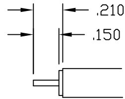
RECOMMENDED CABLE STRIPPING DIM'S
